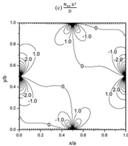
Fig. 3 In-plane stress resultants of a square plate subjected to concentrated in-plane shear loads F_0 at the mid-points of all edges.
