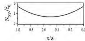
(b) \frac{x}{a} = 0
