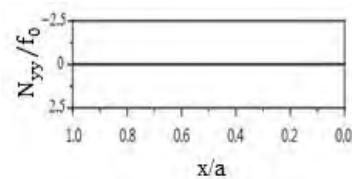
(c) \frac{x}{a} = 0
